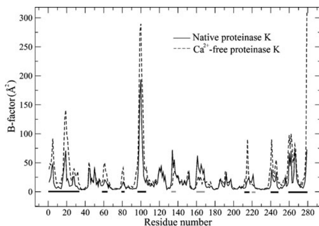
Fig. 2 Comparison of the \text{C}_\alpha B-factors calculated over the 10–50 ns simulations of the native (Solid lines) and \text{Ca}^{2+} -free (dashed lines) proteinases K. The regions exhibiting significant increase and reduction in B-factors upon \text{Ca}^{2+} removal are indicated with black and gray bars along the horizontal axis, respectively
